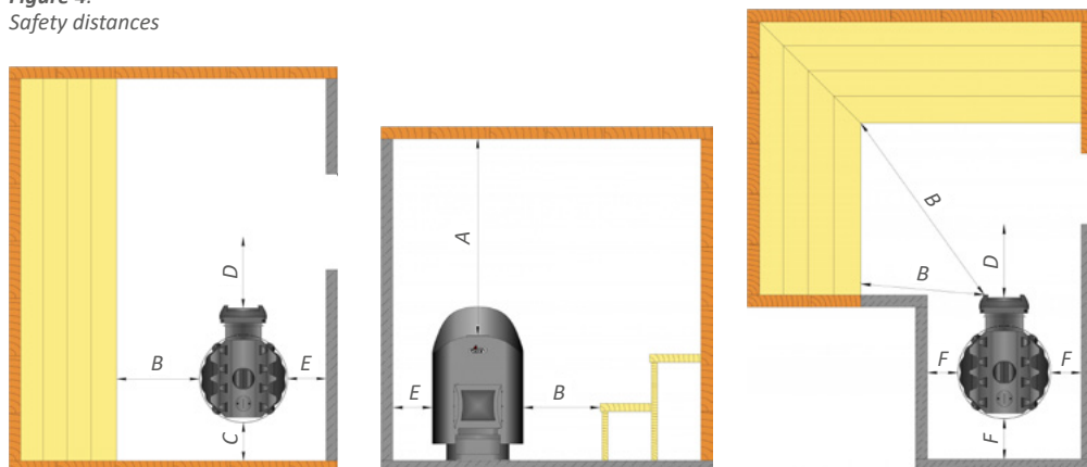
Figure 4. Safety distances
